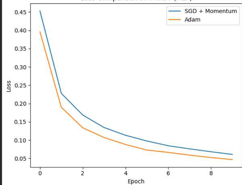
Loss Comparison on MNIST (MLP)
