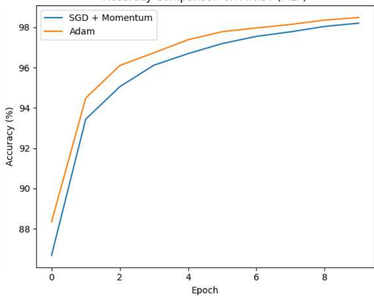
Accuracy Comparison on MNIST (MLP)
